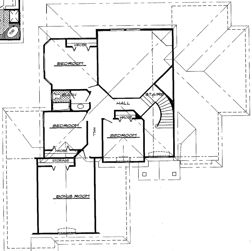
FLOOR PLAN - UPPER
