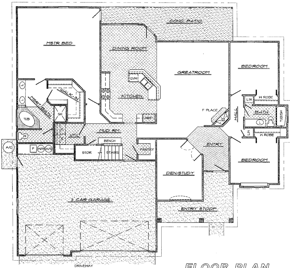
FLOOR PLAN
